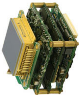
The new MIRICLE® 110KC-25 camera core incorporates a state of the art 25µ lightweight detector
